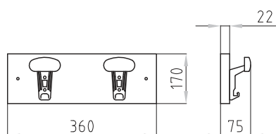
Art. OM 4.382 Attaccapanni 2 posti Clothes-hook 2 places
