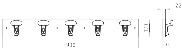
Art. OM 4.383 Attaccapanni 5 posti Clothes-hook 5 places
