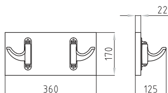
Art. OM 4.388 Attaccapanni 2 posti Clothes-hook 2 places
