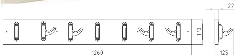
Art. OM 4.390 Attaccapanni 7 posti Clothes-hook 7 places
