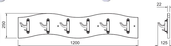
Art. OM 4.391 Attaccapanni sagomato 6 posti Shaped Clothes-hook 6 places
