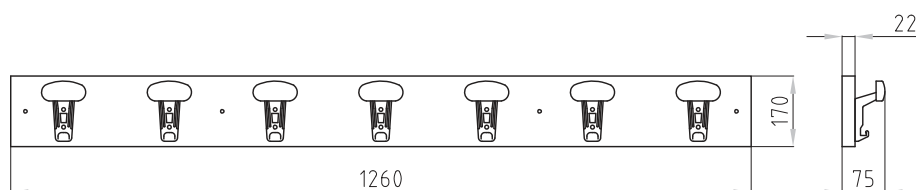
Art. OM 4.384 Attaccapanni 7 posti Clothes-hook 7 places
